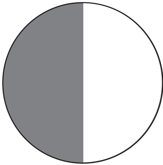
First Quarter
