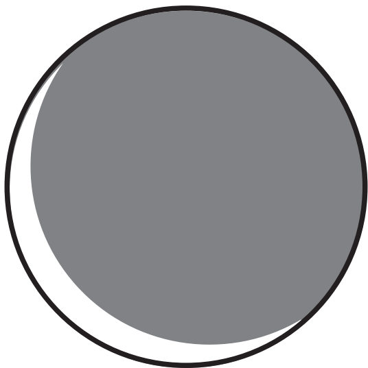
Waning Crescent
