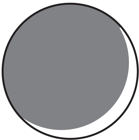
Waxing Crescent
