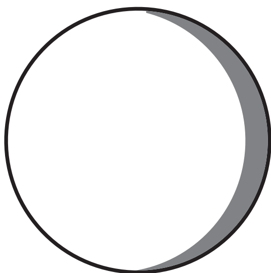
Waning Gibbous
