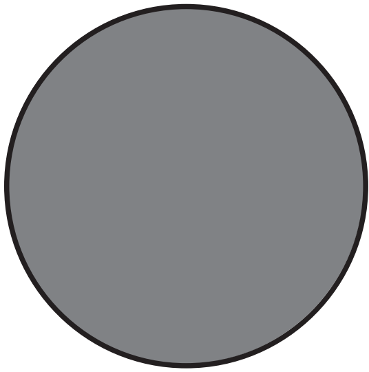
New
