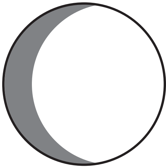
Waxing Gibbous
