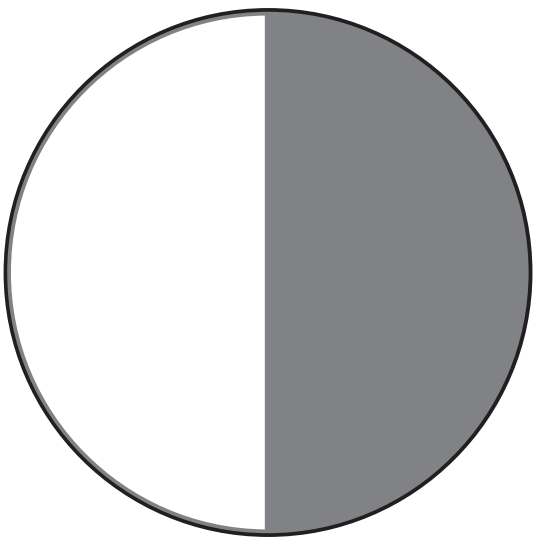
Last Quarter
